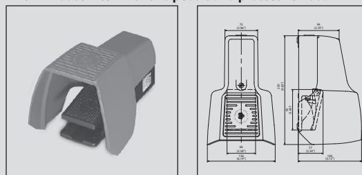
F1 UN – Foot switch with two pedals and protective hood
