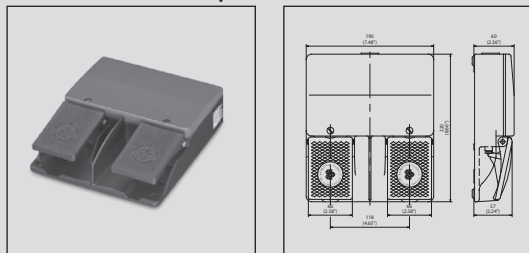
F2 – Foot switch with two pedals
