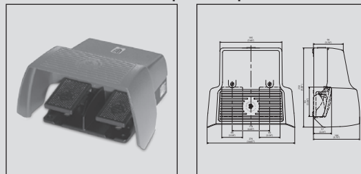
F2 UN – Foot switch with two pedals and protective hood
